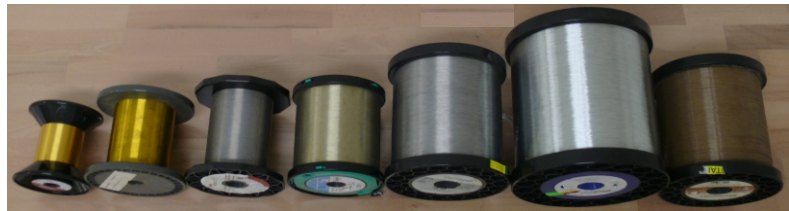
For the wire EDM technology we use \varnothing 0.03mm-0.3mm wires
